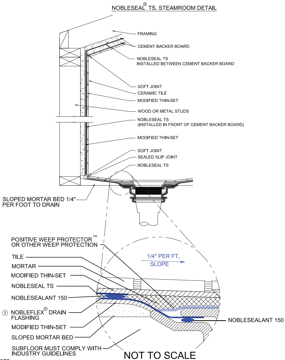
Figure 1. STEAM SHOWER DETAIL
