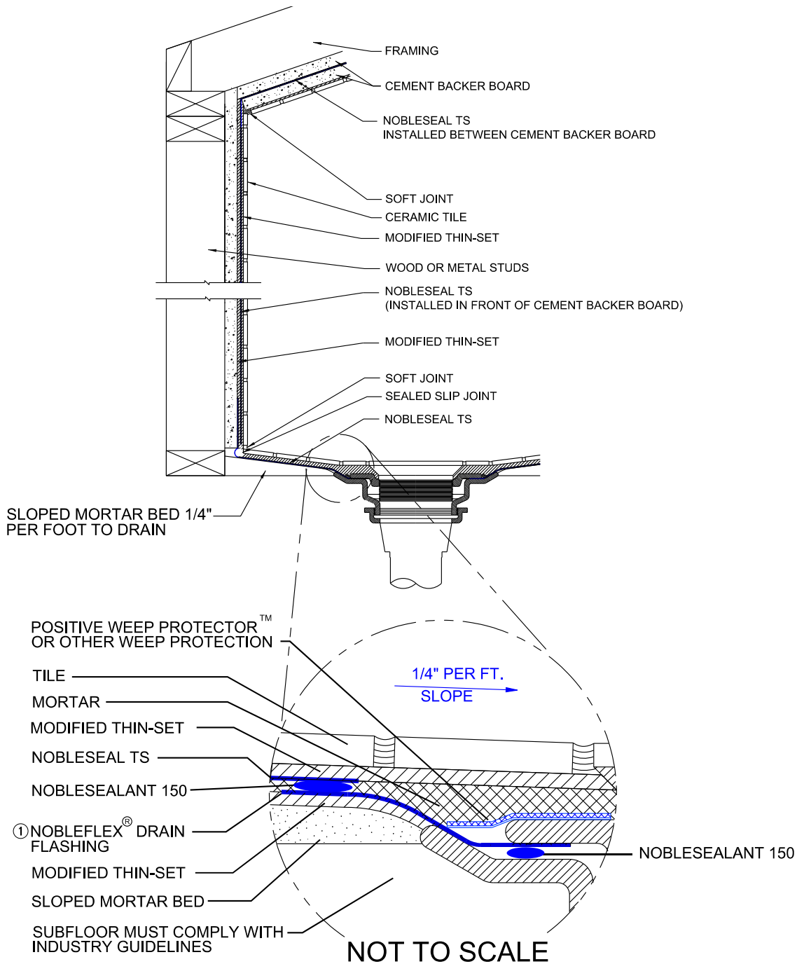
Figure 1. STEAM SHOWER DETAIL
