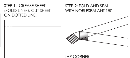
Figure 3. LAP CORNER
