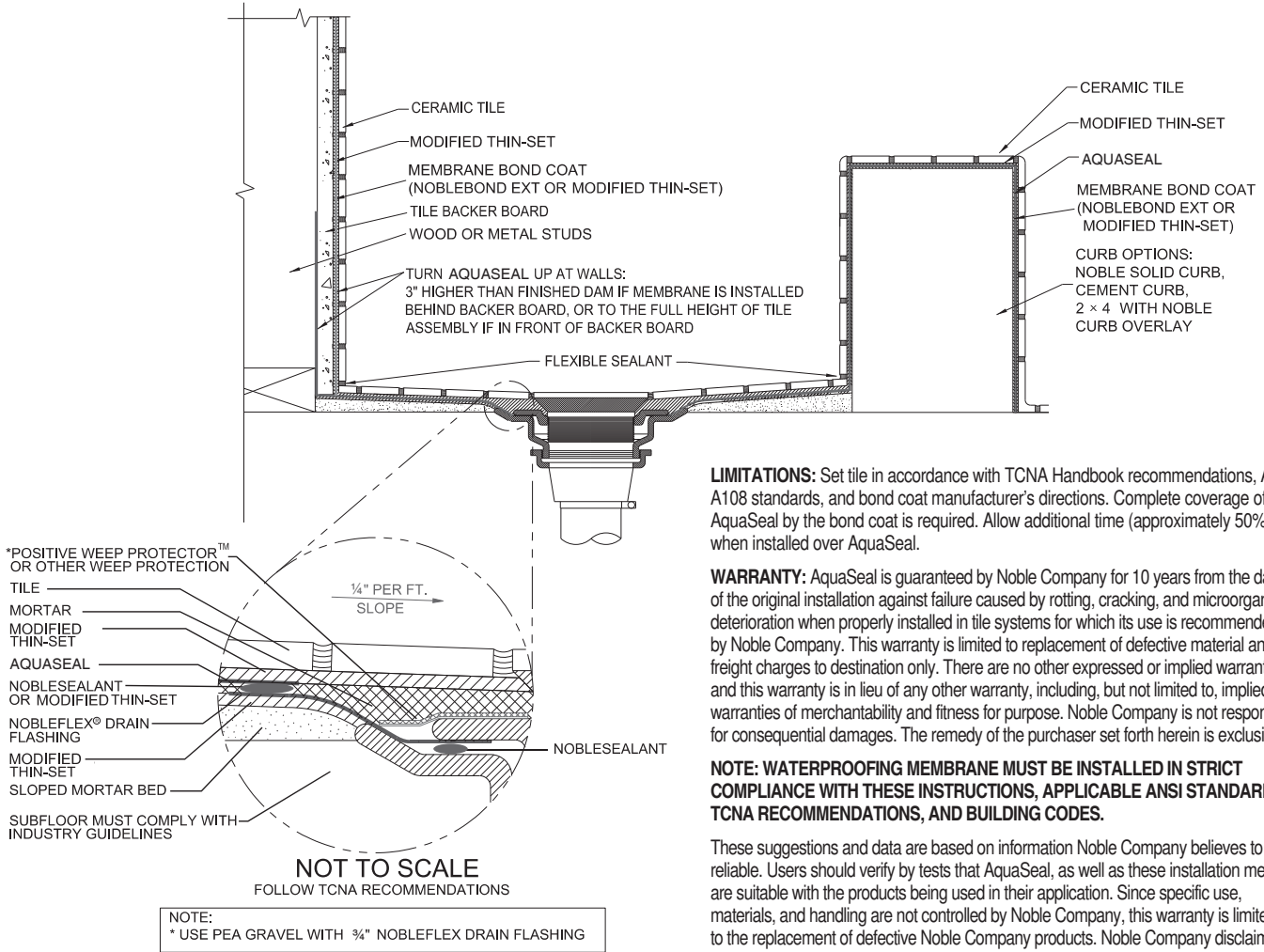
Figure 1. SHOWER DETAIL
