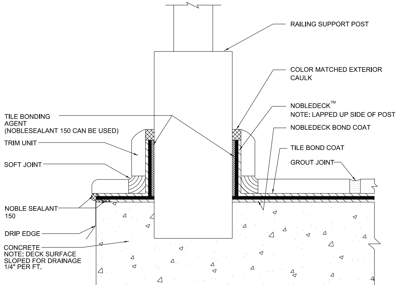
NOBLEDECK POST & EDGE DETAIL
