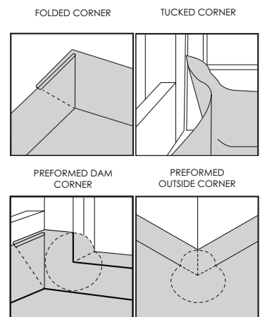
FIGURE 2. CORNERS
